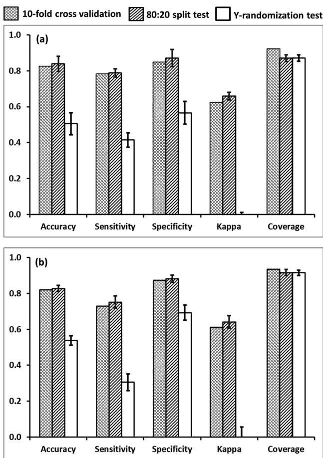
Figure 4. Results of the 80:20 split training/test evaluation and \gamma -randomization tests compared to 10-fold cross-validation: (a) performance measures of RF models for the test set compounds, (b) performance measures of \nu -NN models for the test set compounds. The results are average of 50 runs with the training/test samples randomly selected. The error bars are \pm one standard deviation.
