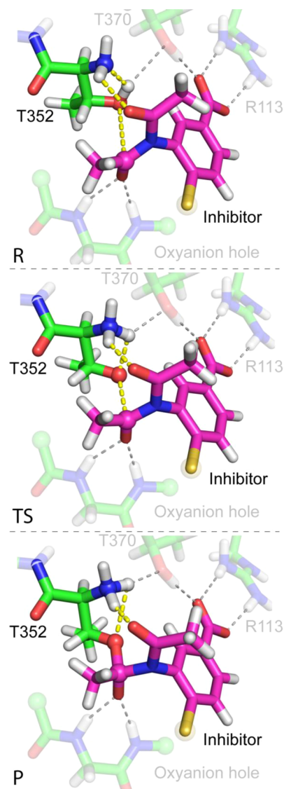
Figure 8. Reactant, transition state, and product for the formation of the tetrahedral intermediate of CapD with covalent inhibitor capsidin. Snapshots of the changes in the QM region of the ONIOM(QM/MM) system along the reaction path. Enzyme carbon atoms are colored green, while inhibitor carbon atoms are colored magenta. Hydrogen, nitrogen, oxygen, and sulfur atoms are colored white, blue, red, and yellow, respectively. Hydrogen bonds between the ligands and the enzyme are shown as dashed gray lines. Dashed yellow lines connect the atoms that are involved in the chemical transformations. The residues of the active site that are not directly involved in the reaction are shown in faded, transparent colors. Atoms that link the QM region to the rest of the system described by molecular mechanics are depicted with transparent spheres around them. These atoms are substituted for hydrogen atoms, and their bond lengths are adjusted accordingly during QM calculations.
