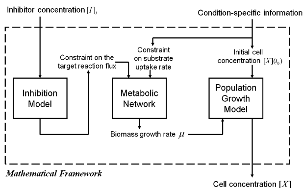
Fig. 1 Mathematical framework: a set of coupled models used to simulate an inhibitor's effect on the growth of bacteria in host cells. Given the inhibitor concentration [I]_i , the inhibition model describes how the inhibitor affects the flux of the reaction(s) being inhibited [i.e., the target reaction(s)]. These effects are modeled via explicit constraints on the target reaction flux(es). Using these constraints and constraints on the substrate uptake rates, we analyzed the metabolic network to infer the biomass production rate \mu . Using the population growth model, we related the biomass production rate \mu to cell concentration [X] . Once these model components were specified, together with the constraints on the substrate uptake rates and the initial cell concentrations [X](t_0) in host cells, the calculations performed within this framework only required input in the form of a specific inhibitor concentration [I]_i to predict cellular growth. Here, the inhibitor concentration [I]_i indicates the concentration of the inhibitor inside the macrophage and the subscript "i" denotes intracellular concentration.
