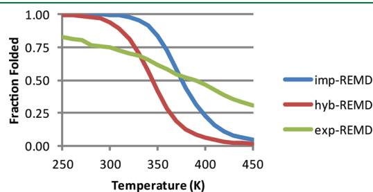
Figure 6. Simulated melting curves from the implicit, hybrid, and explicit REMD methods.
